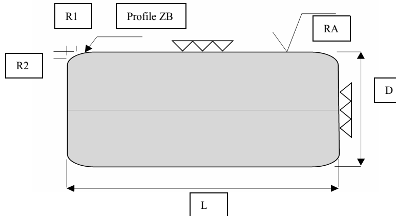
Rollers nominal dimensions
