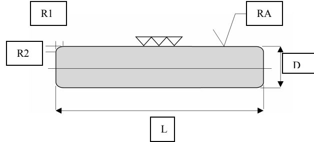
Needle rollers nominal dimensions
