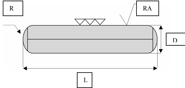
Needle rollers nominal dimensions
